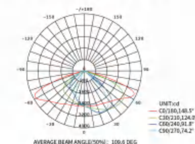
Meridian Light Distribution Curve(60W Parameter)
